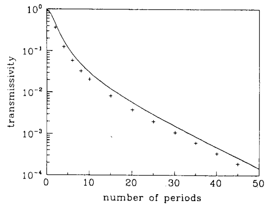
FIG. 2. Transmissivity following from envelope-function approach (solid line) compared to results from exact calculations (crosses), for linear stack with varying number of periods. For this example, n_1 = 2.0 , n_2 = 3.0 , and d_1 = d_2 = 0.5 \mu\text{m} . The wave number in the surrounding medium k_s = 1.10333 \mu\text{m}^{-1} .
