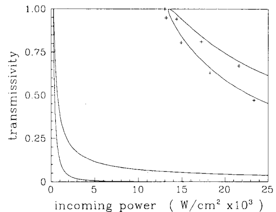
FIG. 6. Transmissivity vs incoming power S_0 , for nonlinear stack with n_1=1.9 , n_2=2.1 , d_1=d_2=0.1 \mu\text{m} , \chi^{(3)}=-10^{-6} e.s.u. uniformly, and a length of 200 stack periods. Furthermore, k_s=7.62500 \mu\text{m}^{-1} .
