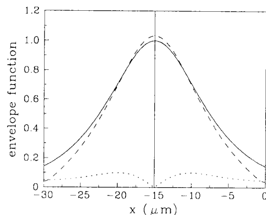
FIG. 4. Profiles of the envelope functions associated with the principal term (dashed line) and companion term (dotted line), compared to that of the soliton solution (solid line). For this example, the nonlinear stack has a uniform \chi^{(3)} = -10^{-6} e.s.u. Furthermore, n_1 = 1.9 , n_2 = 2.1 , d_1 = d_2 = 0.1 \mu\text{m} , and k_s = 7.6200 \mu\text{m}^{-1} . The Poynting vector is chosen such that the envelope function has a period of 150 stack periods.
