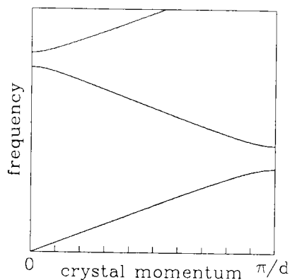
FIG. 1. Schematic of dispersion curve of a periodic dielectric stack in the reduced zone scheme.
