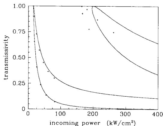
FIG. 5. Transmissivity vs incoming power S_0 , for nonlinear stack with n_1=2.0 , n_2=3.0 , d_1=d_2=0.5 \mu\text{m} , \chi^{(3)}=-10^{-4} e.s.u. uniformly, and a length of 80 stack periods. Furthermore, k_s=1.10333 \mu\text{m}^{-1} .
